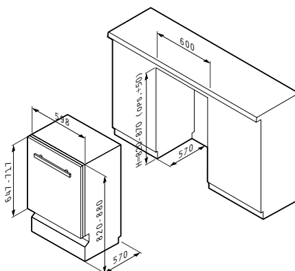
Dishwasher DWE 60FI - 033000605
