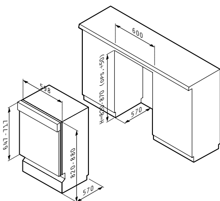
Dishwasher DWG 60SI - 033000805
