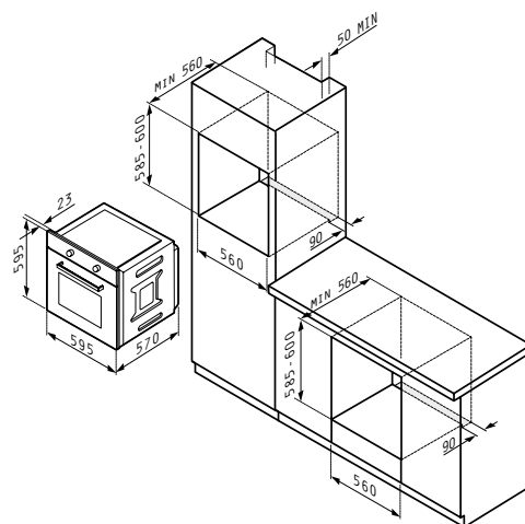
Oven Rustic Beige Metal 733070 - 034068201 Oven Rustic Black Metal 733070 - 034068301
