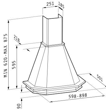
Rustic Chimney 60cm - 065018002 Rustic Chimney 90cm - 065018102
