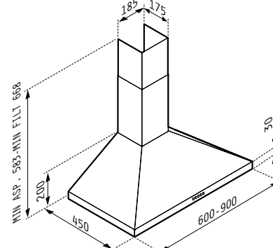
Square Chimney Black 60cm - 065040401 Square Chimney Black 90cm - 065040501
