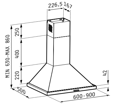
Square Chimney Ecoline 60cm - 065030801 Square Chimney Ecoline 90cm - 065030901
