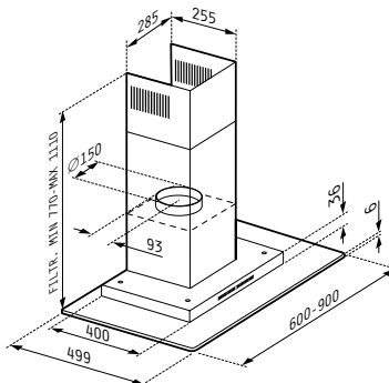
Cielo 60cm - 065036501 Cielo 90cm - 065036601
