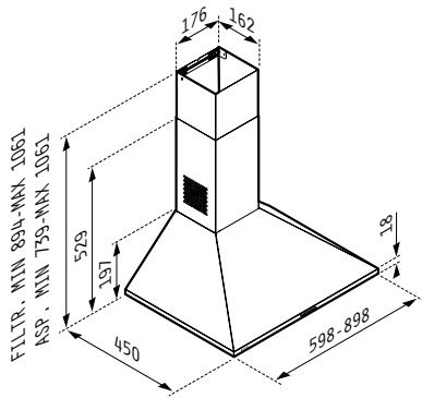
Square Chimney Lux 60cm - 065030102 Square Chimney Lux 90cm - 065030202
