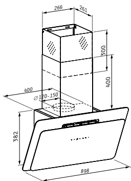
Vetrio Black Glass 60cm - 065039301 Vetrio Black Glass 90cm - 065039601
