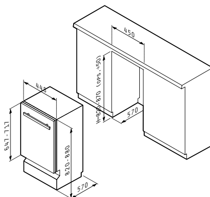
Dishwasher DWF 45FI - 033000705
