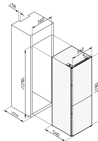
Built-In Combi Refrigerator BIR 178 - 031007701
