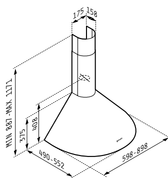
Round Chimney 60cm - 065017801 Round Chimney 90cm - 065017901
