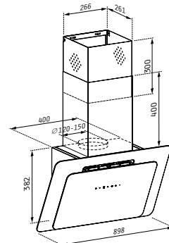
Vetrio White Glass 60cm - 065039201 Vetrio White Glass 90cm - 065039501
