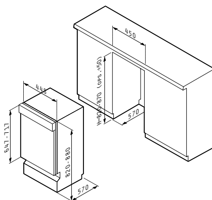
Dishwasher DWH 45SI - 033000905
