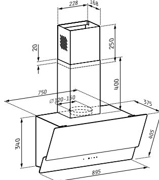
Livelo Black Glass 60cm Ecoline - 065038801 Livelo Black Glass 90cm Ecoline - 065038901
