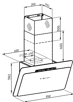
Vetrio Grey Glass 60cm - 065039401 Vetrio Grey Glass 90cm - 065039701
