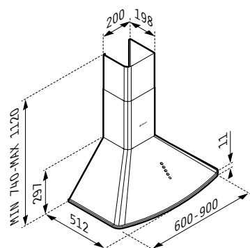
Oval Chimney 60cm - 065030401 Oval Chimney 90cm - 065030501
